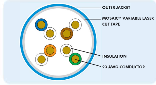
Cat 6A Cross-Section
