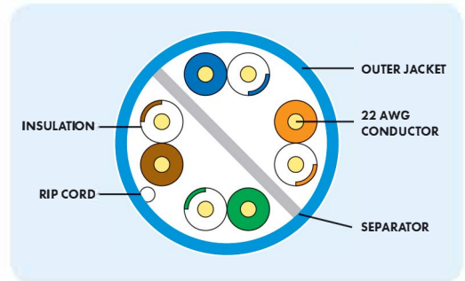
Cat 6 (22 AWG) Cross-Section
